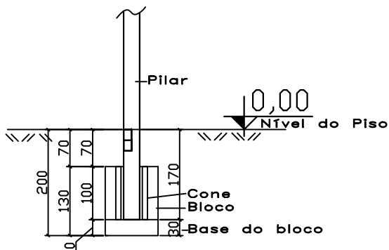
COTAS P11-P24,P32-P44
